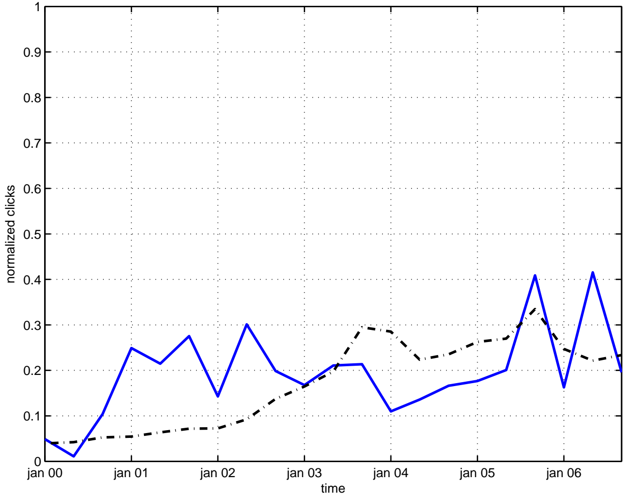
asymptotic freedom
