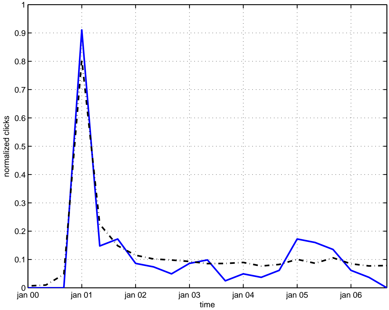
asymptotic behavior zero mode
