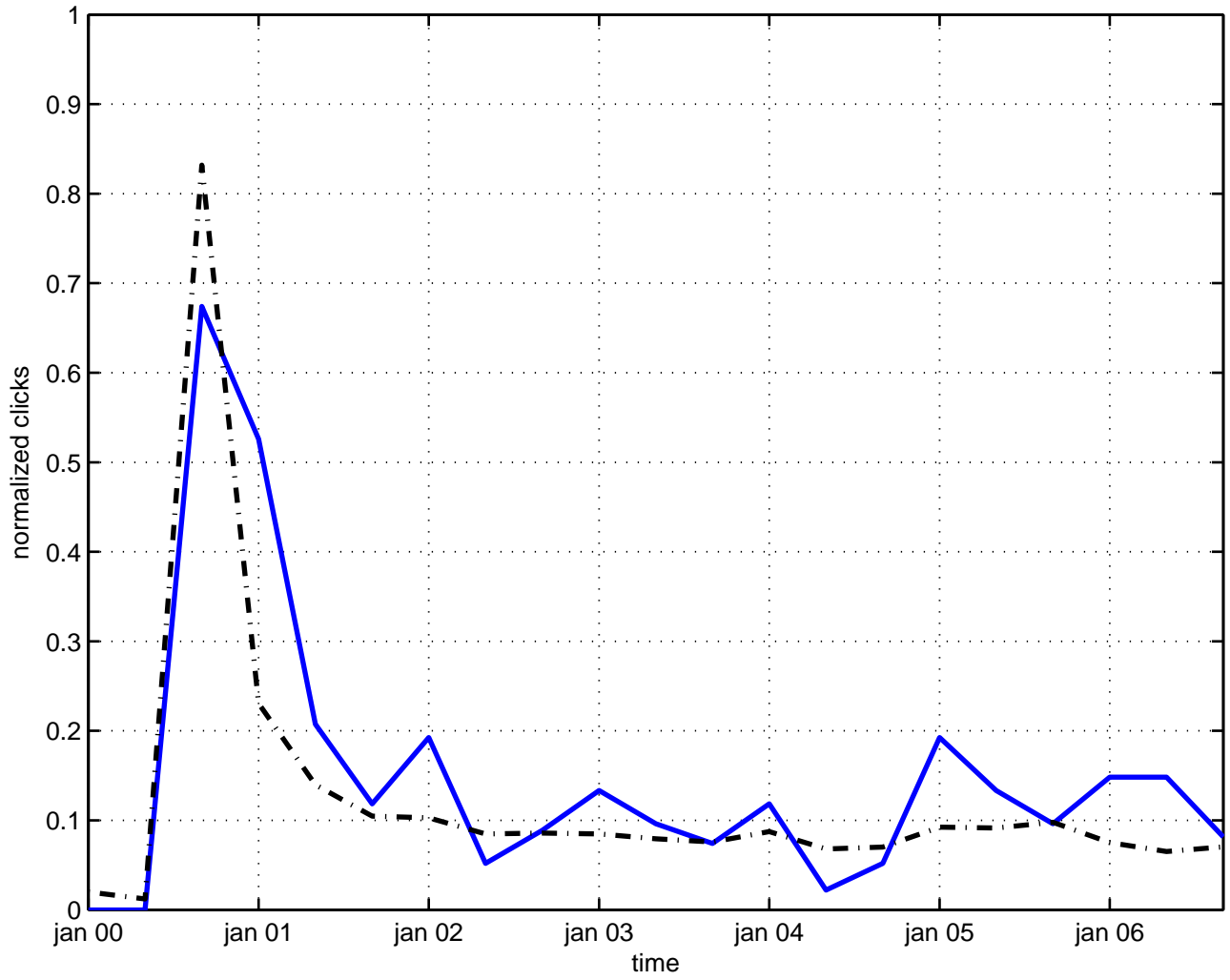
asymptotic behavior topology
