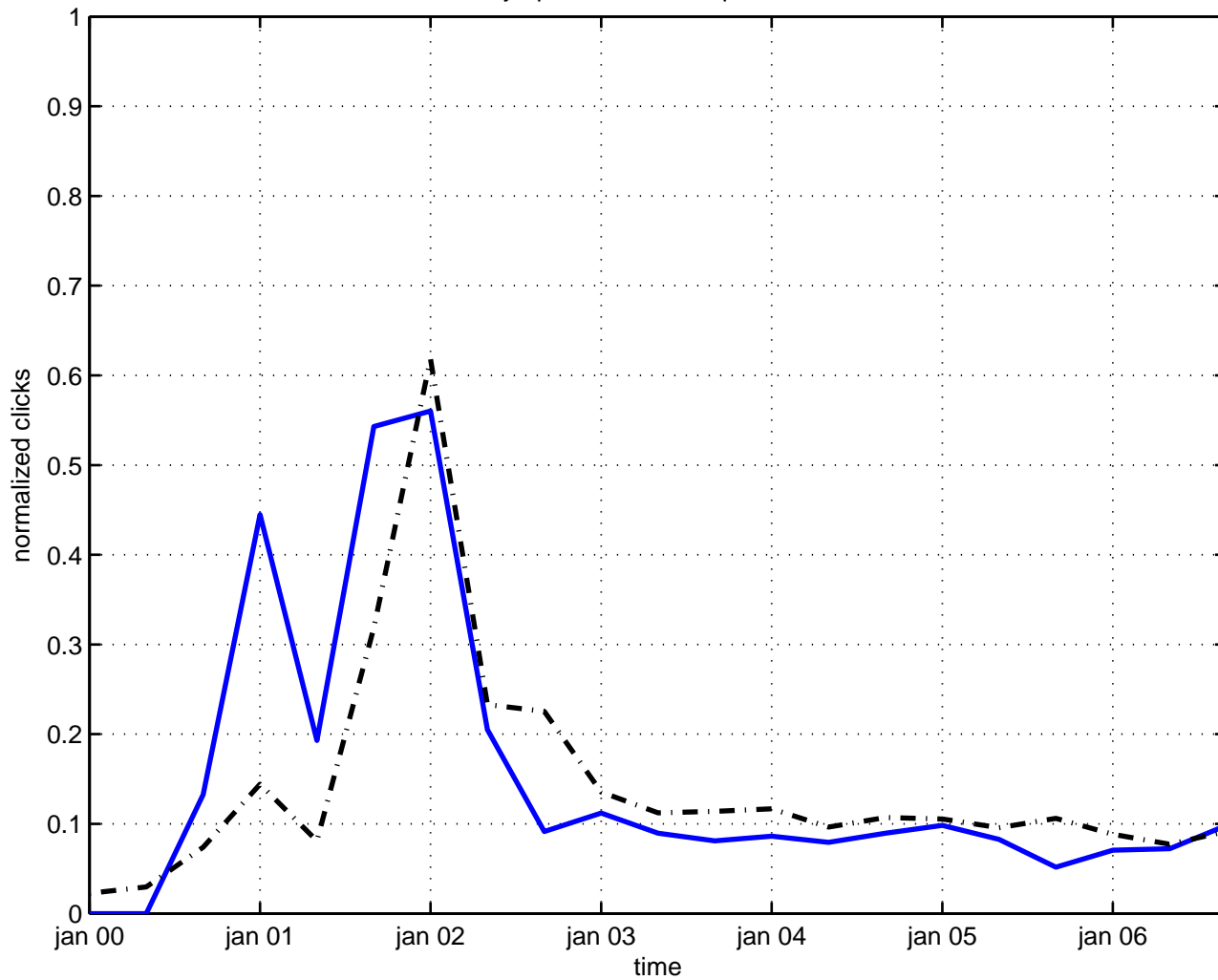
asymptotic behavior space-time
