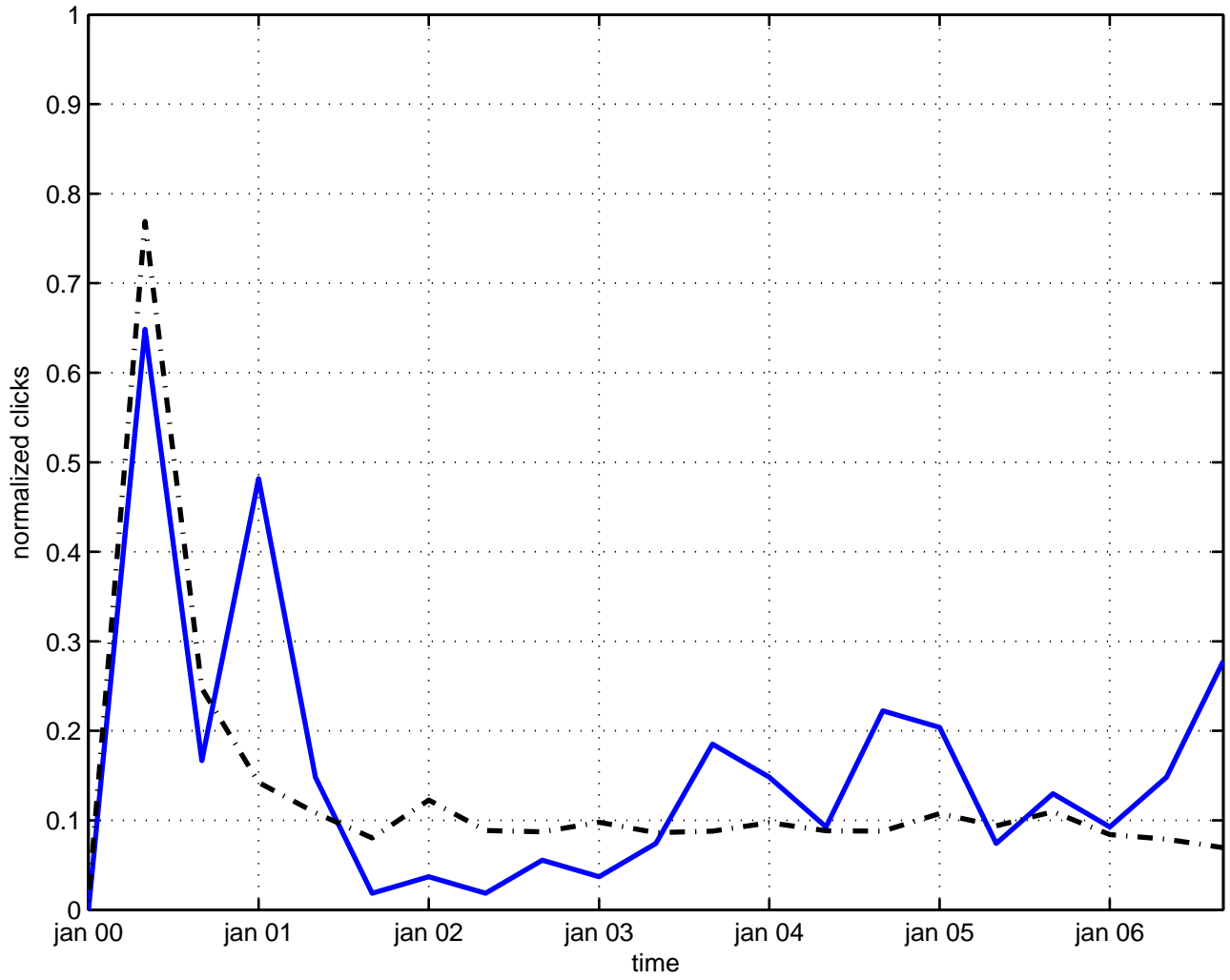
asymptotic behavior monodromy
