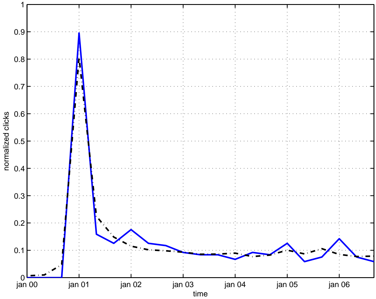
asymmetry time reversal
