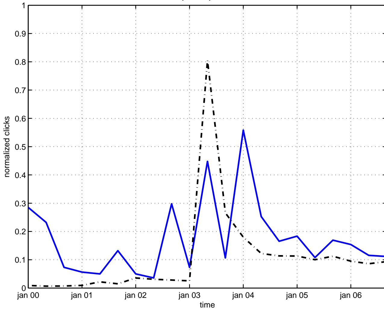
asymmetry orbifold
