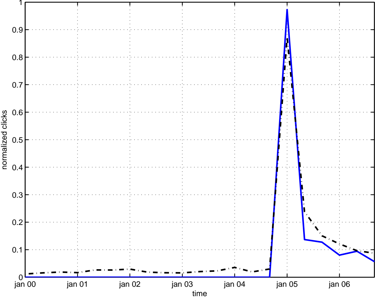
asymmetry compactification
