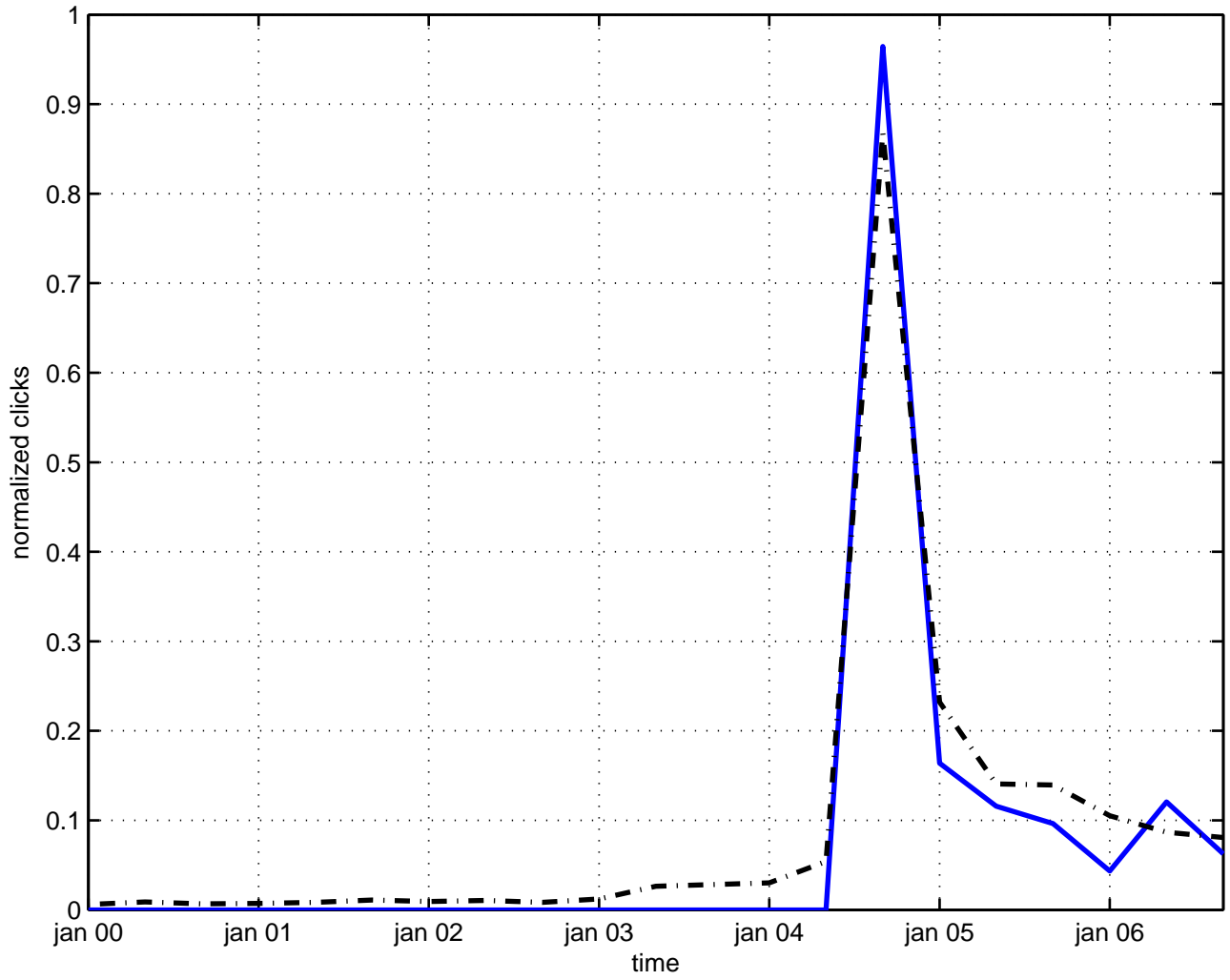
asymmetry antimatter
