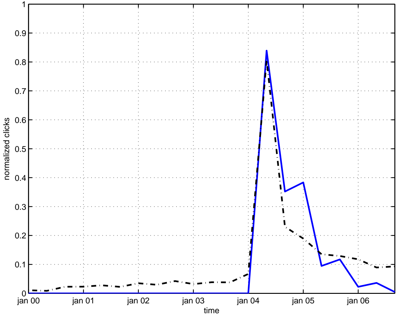
associated production higgs particle
