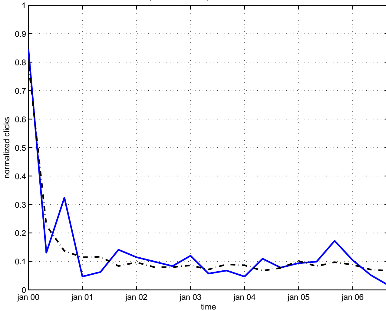
any-dimensional quantum mechanics
