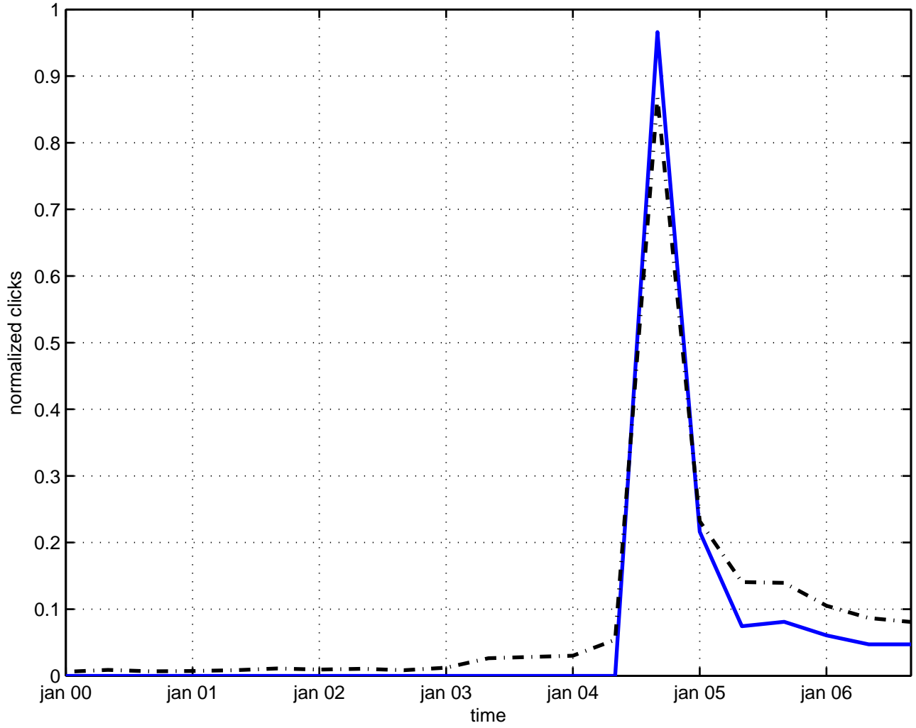
any-dimensional gauge field theory
