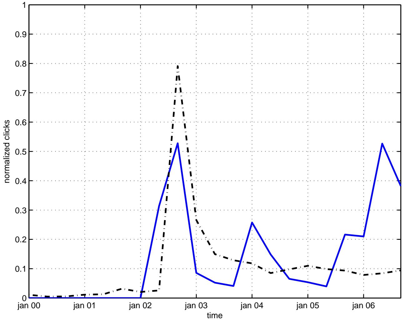
antiparticle
