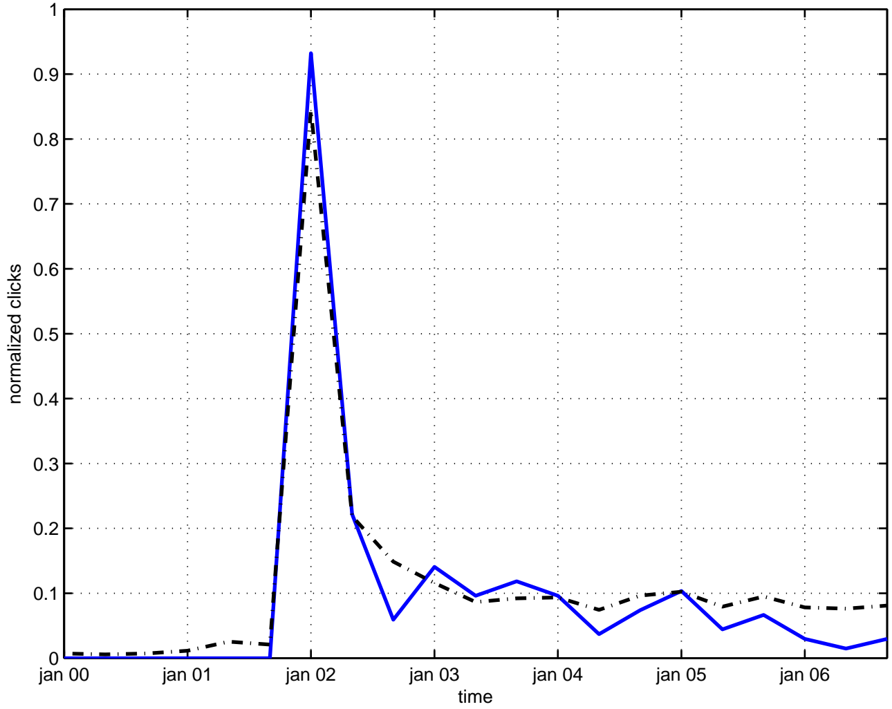
antiparticle ghost
