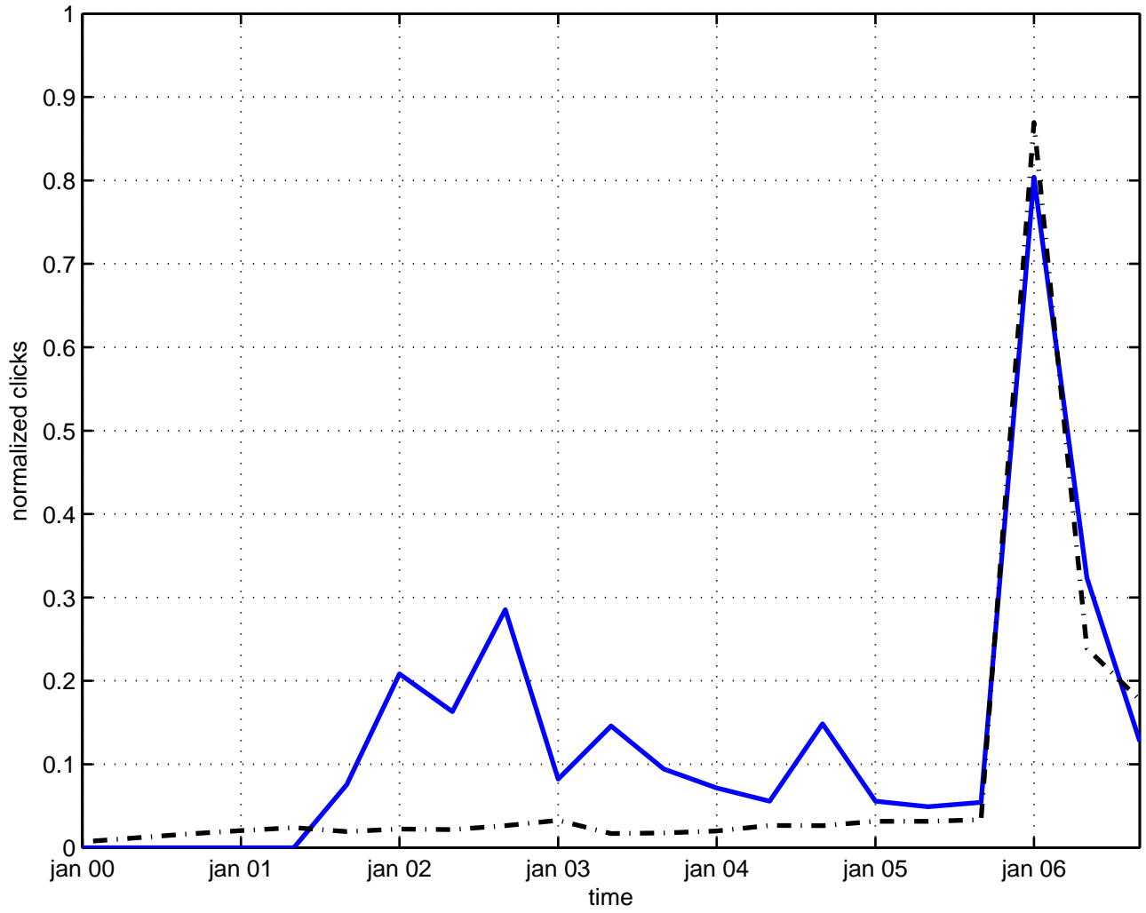
antiferromagnet
