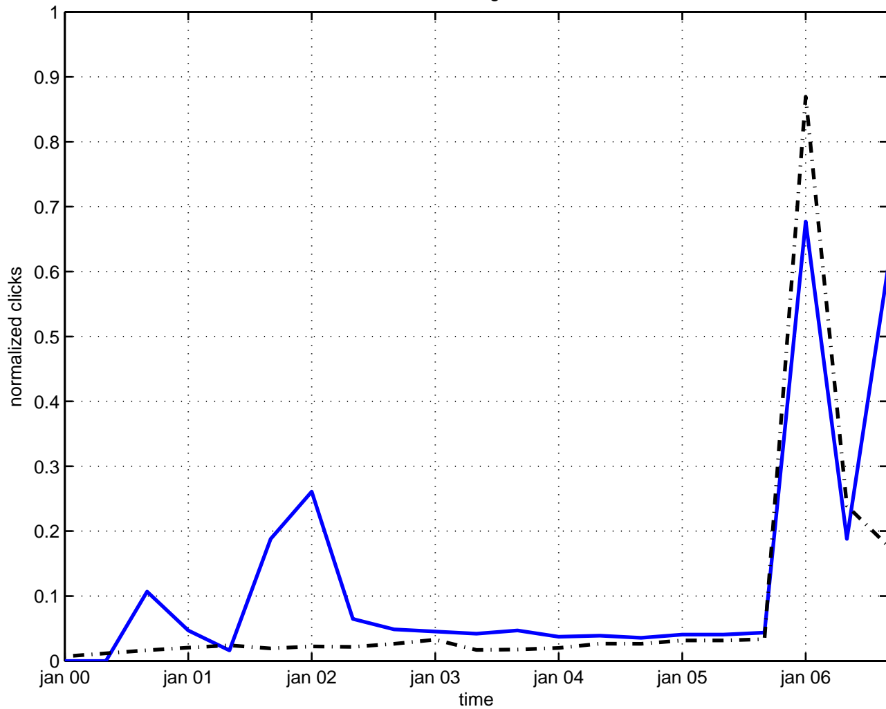
anti-de sitter gravitation
