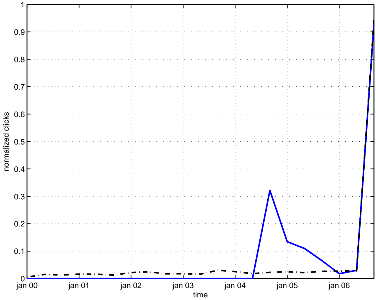
anti-de sitter bubble
