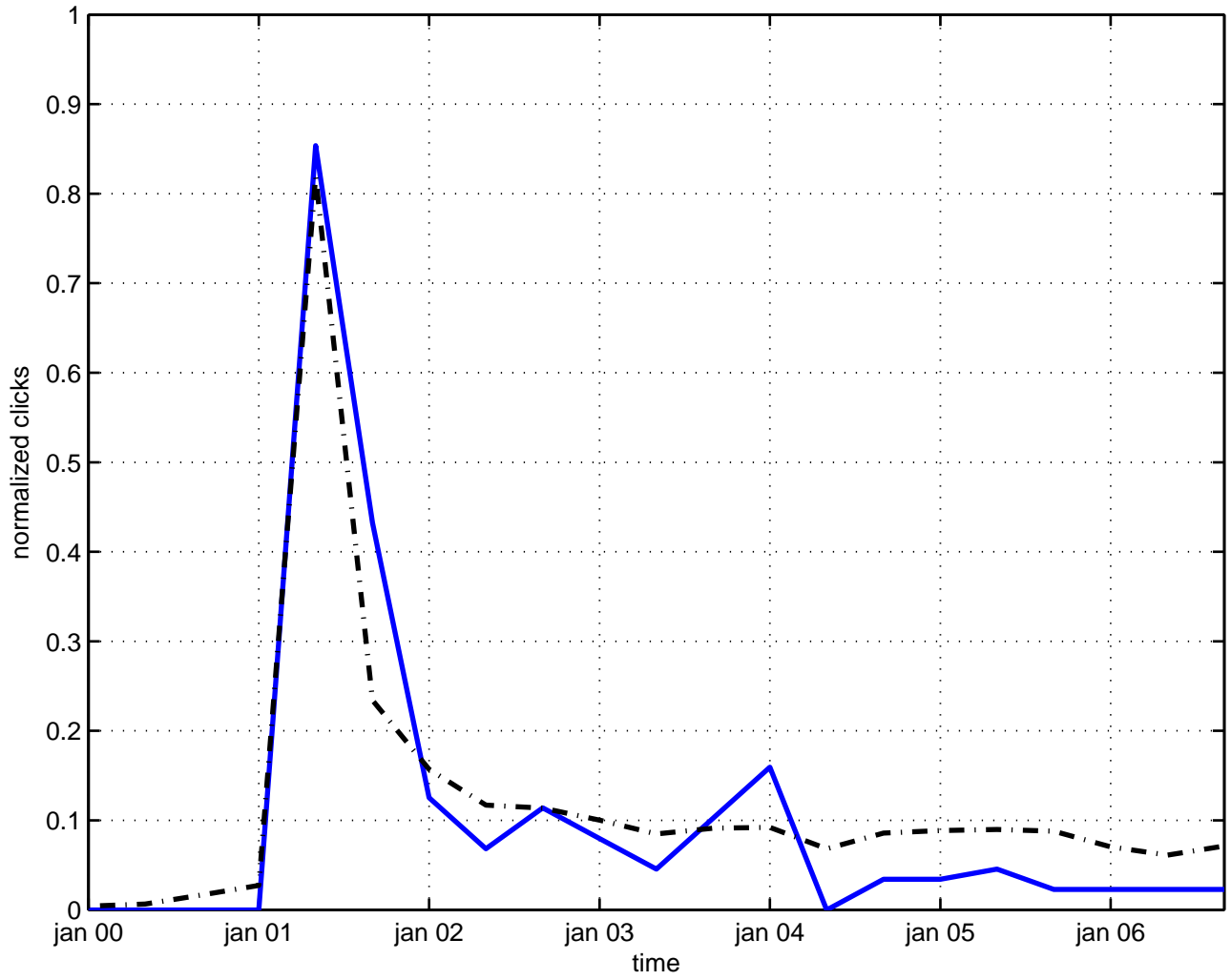
anomaly sum rule
