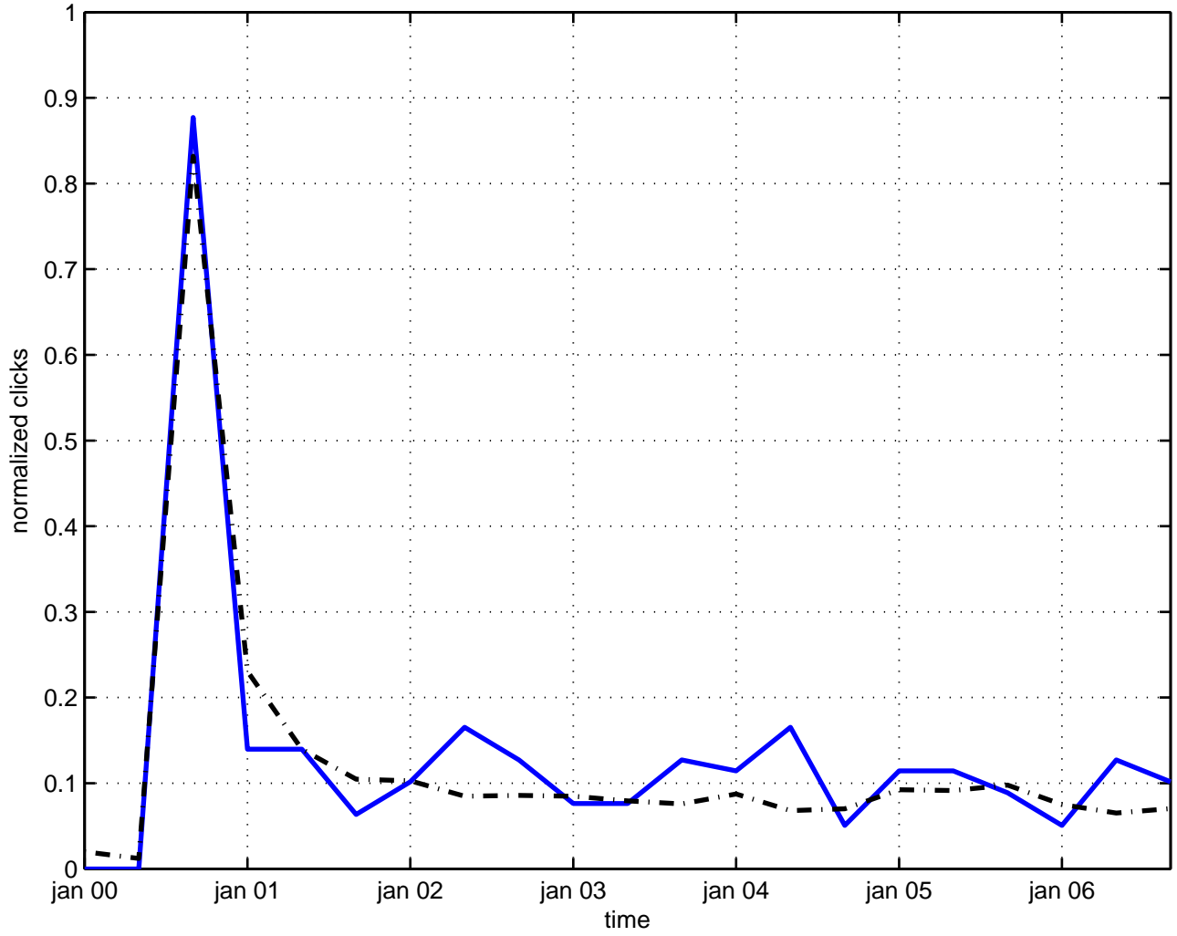
anomaly space-time
