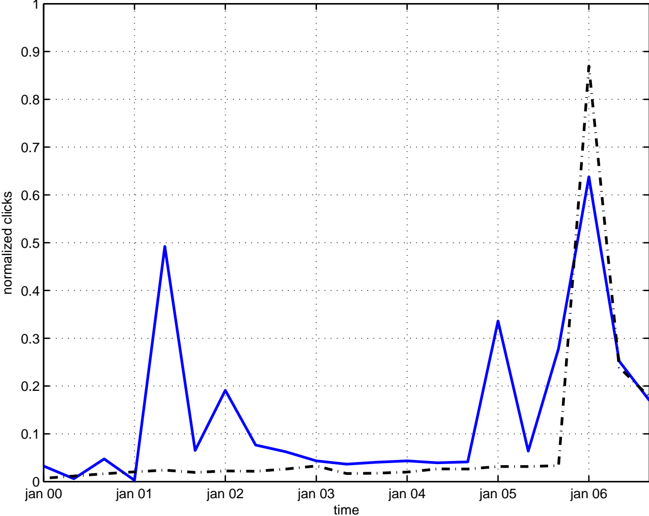
anomaly gravitation
