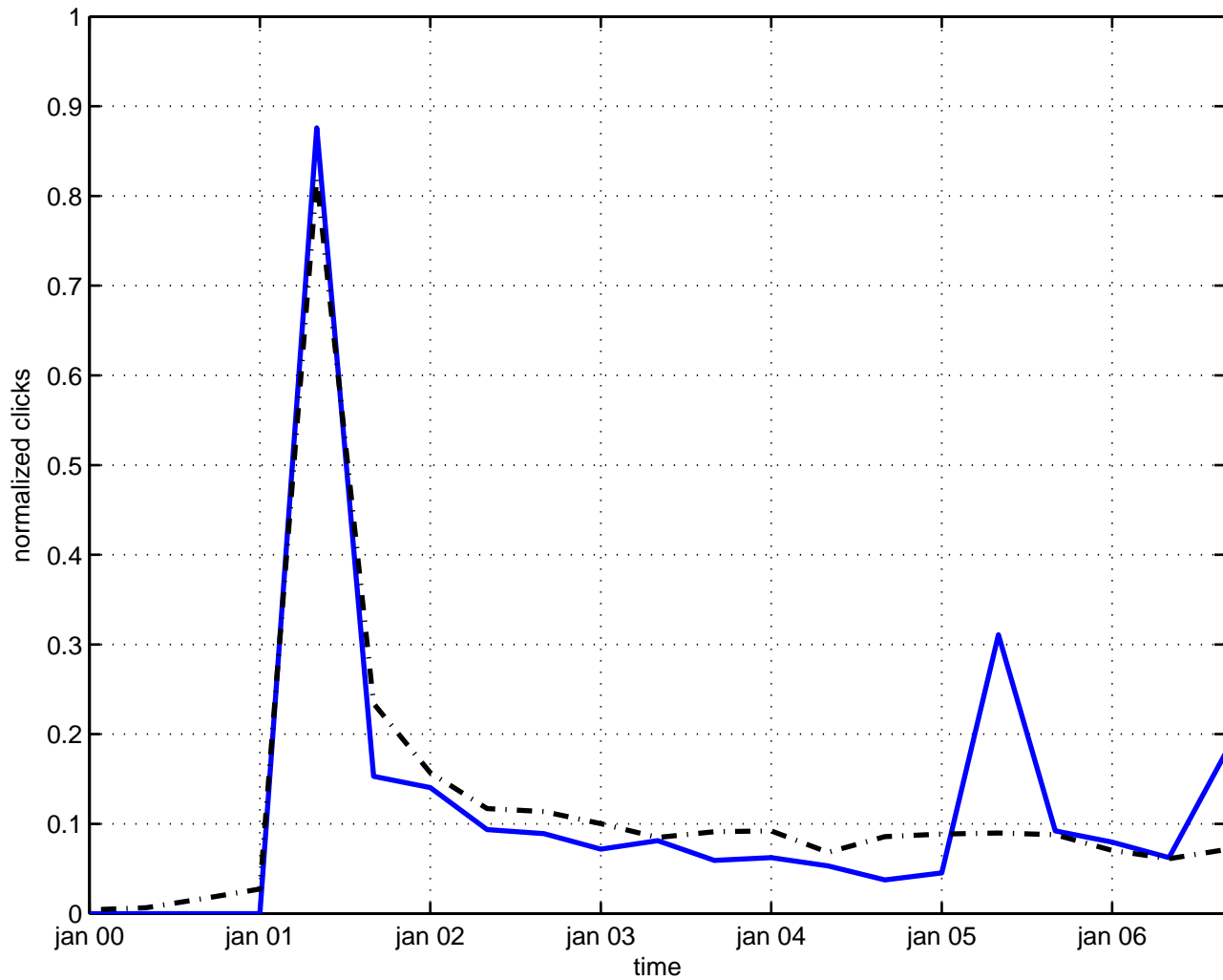
annihilation
