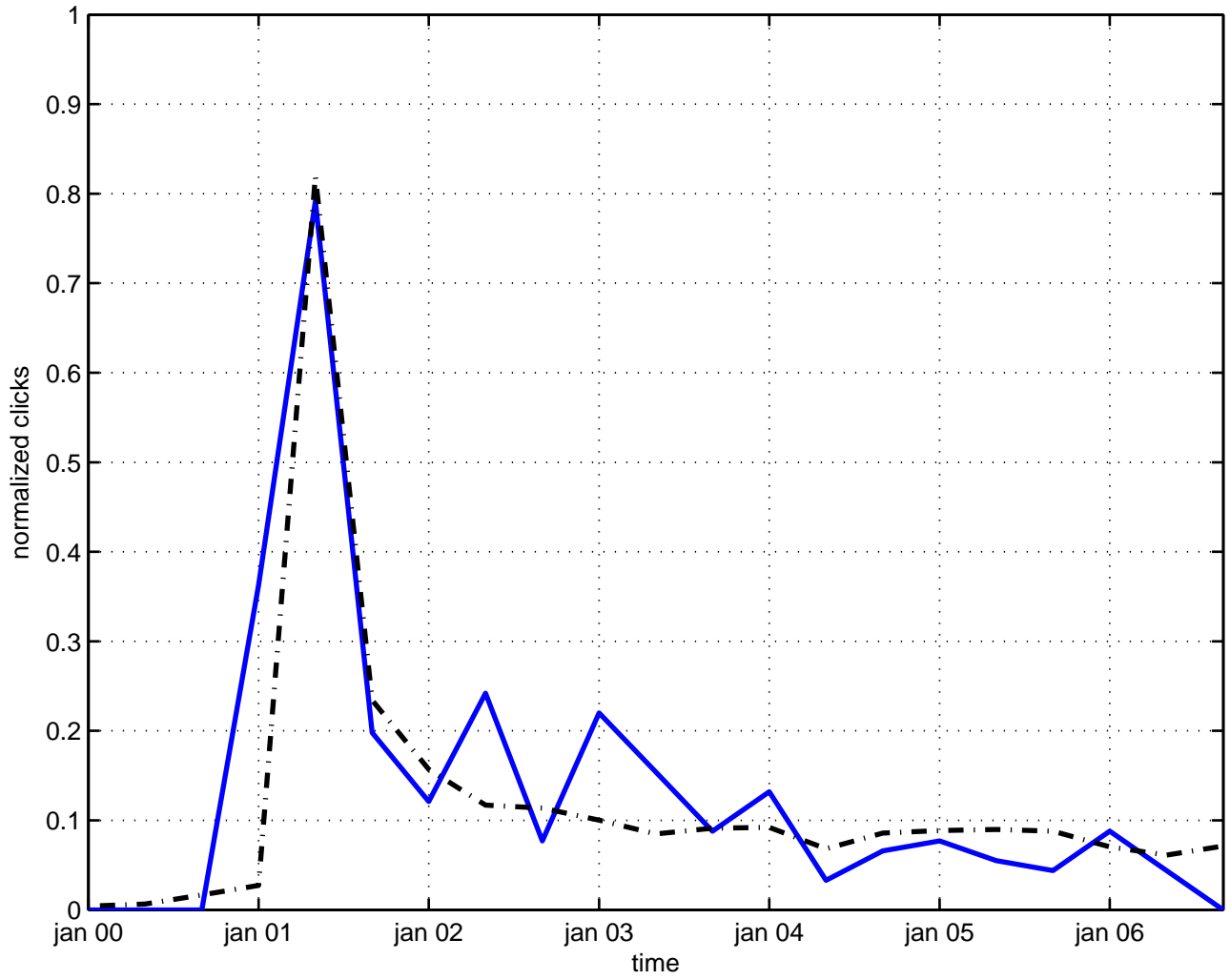
annihilation photon photon
