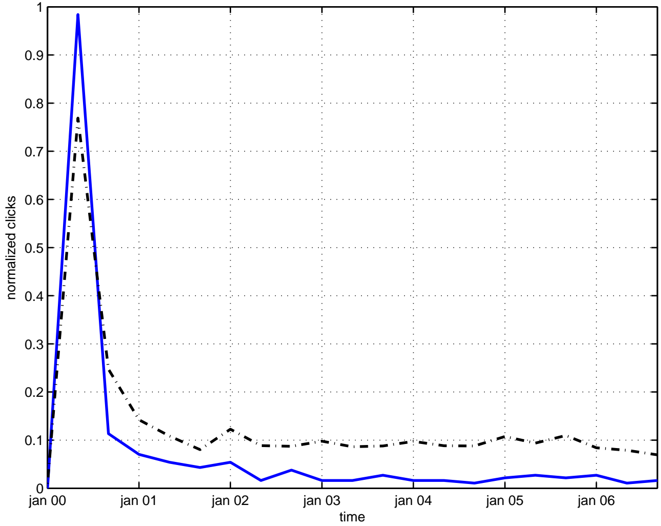
annihilation membrane model
