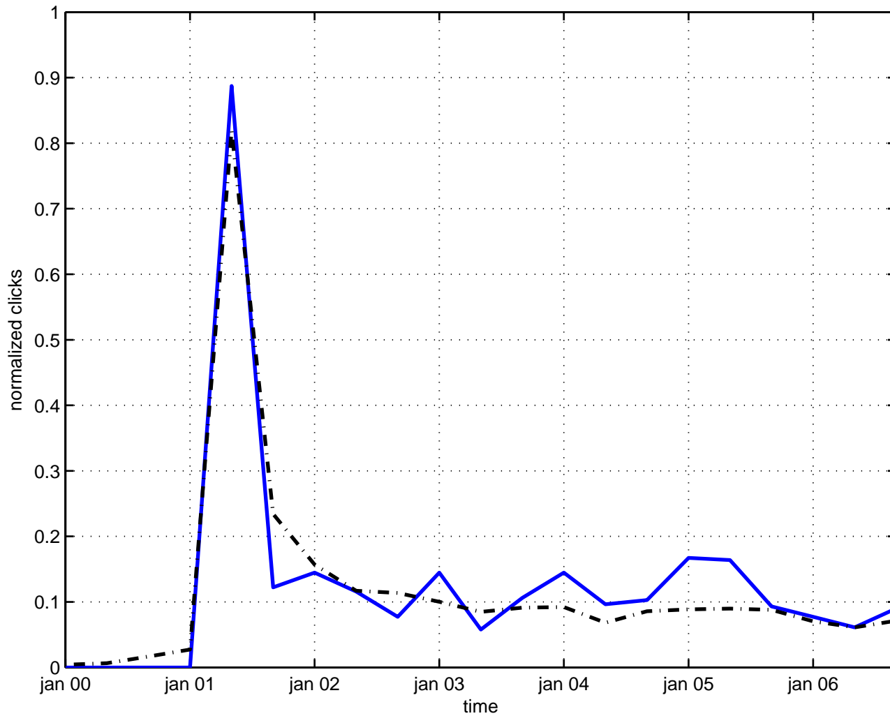
annihilation d-brane
