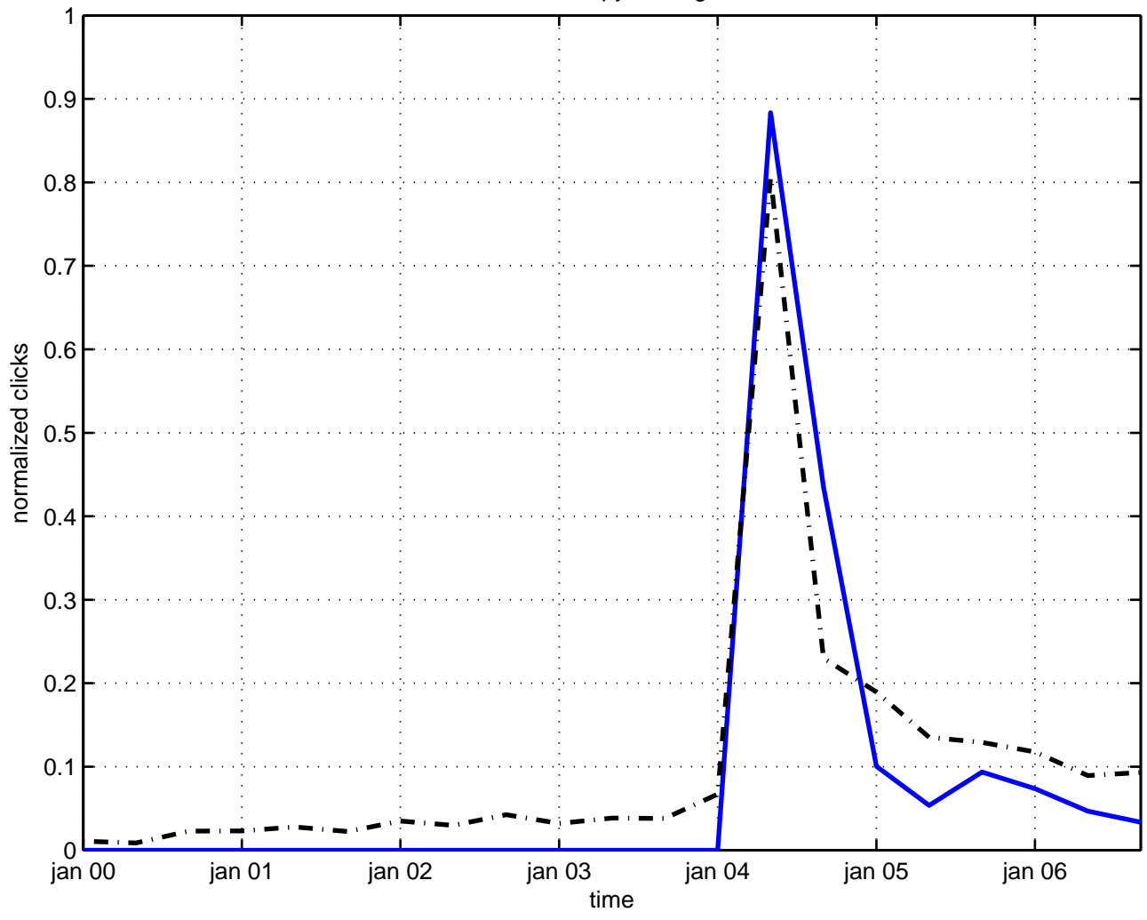
anisotropy scaling
