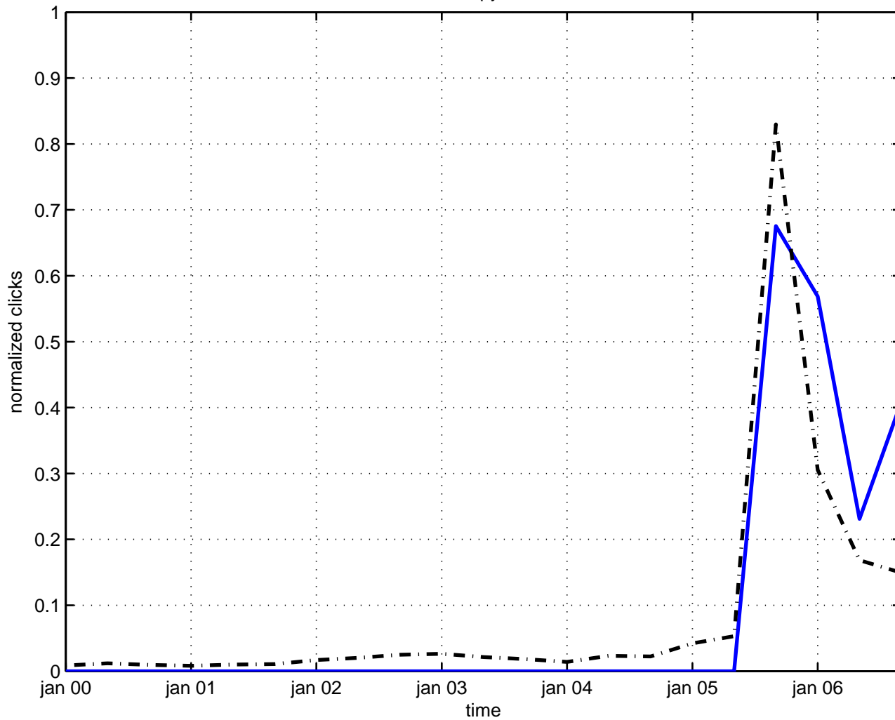
anisotropy lattice
