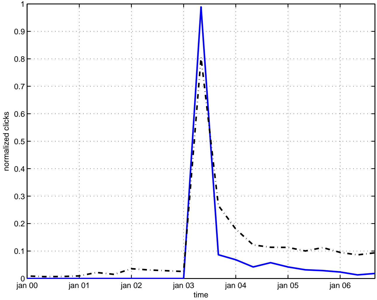
anisotropy inflation
