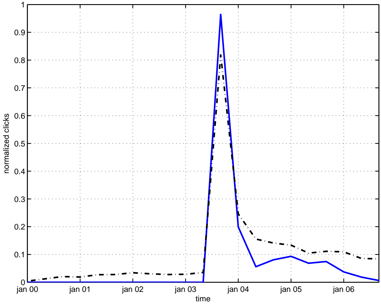
algebra space-time
