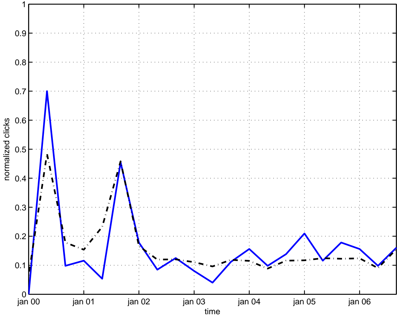
algebra quantization
