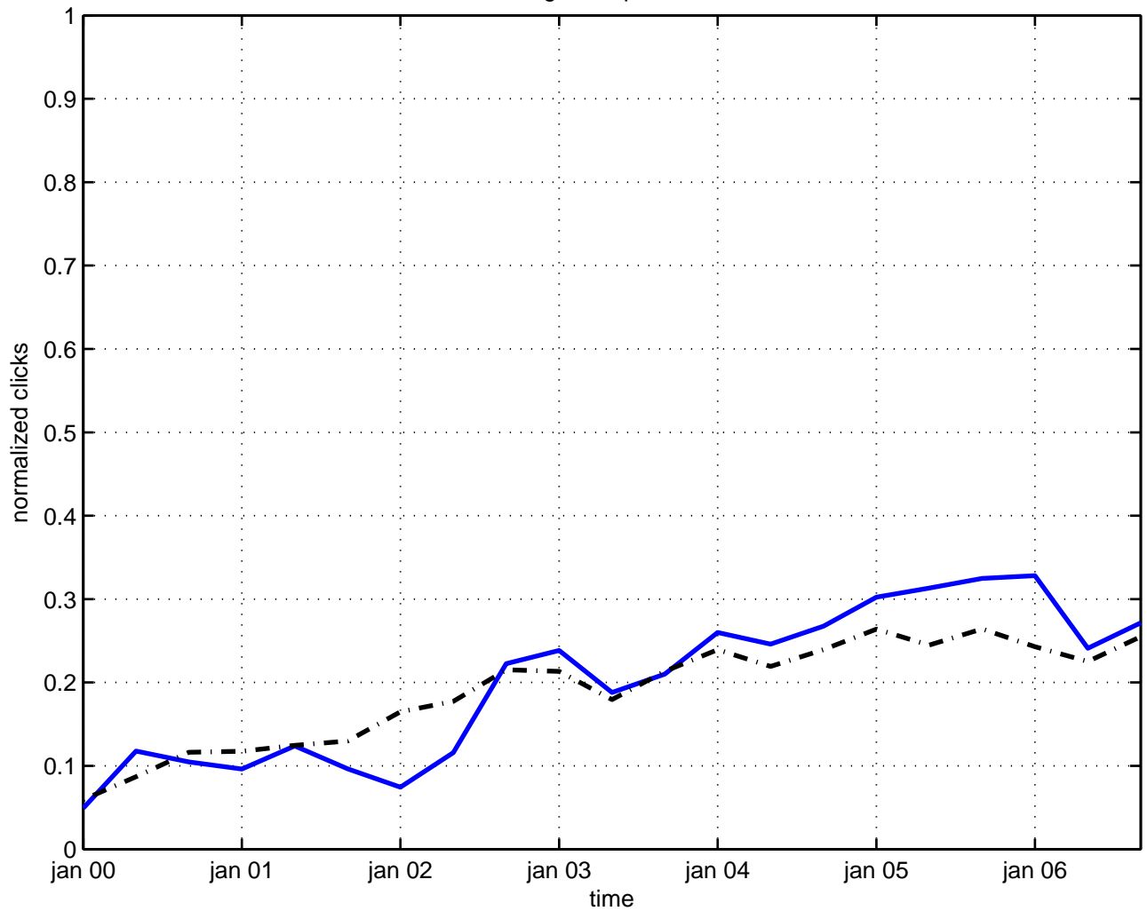
algebra operator
