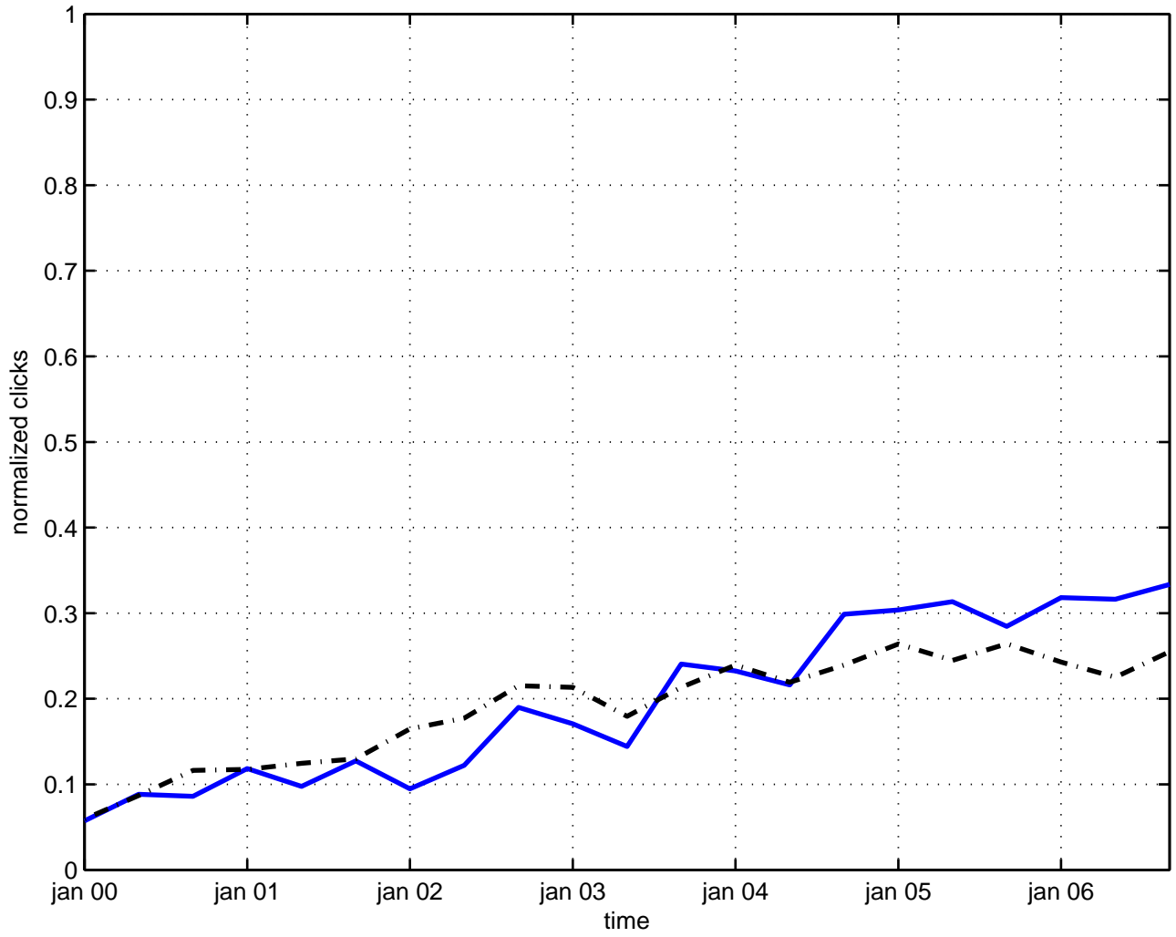
algebra geometry
