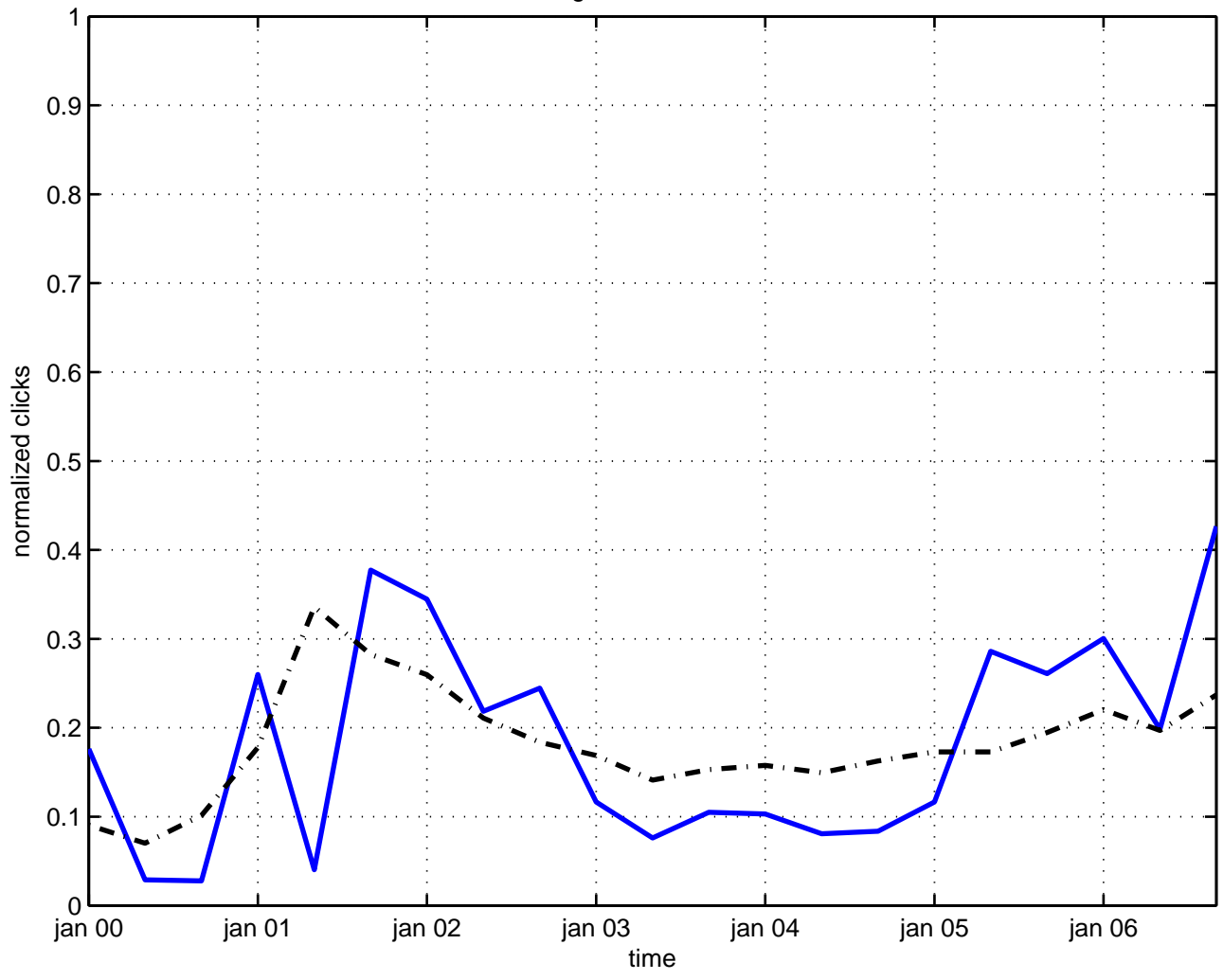
algebra constraint
