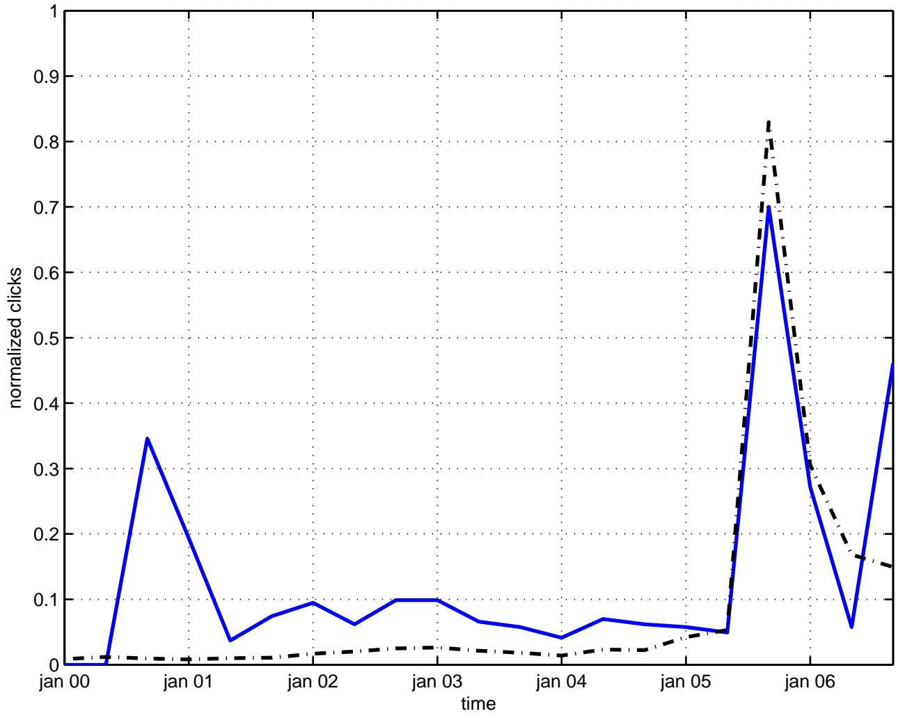
algebra charge
