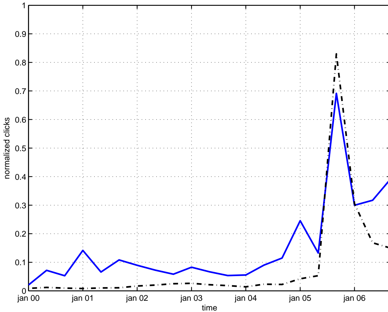
aharonov-bohm effect
