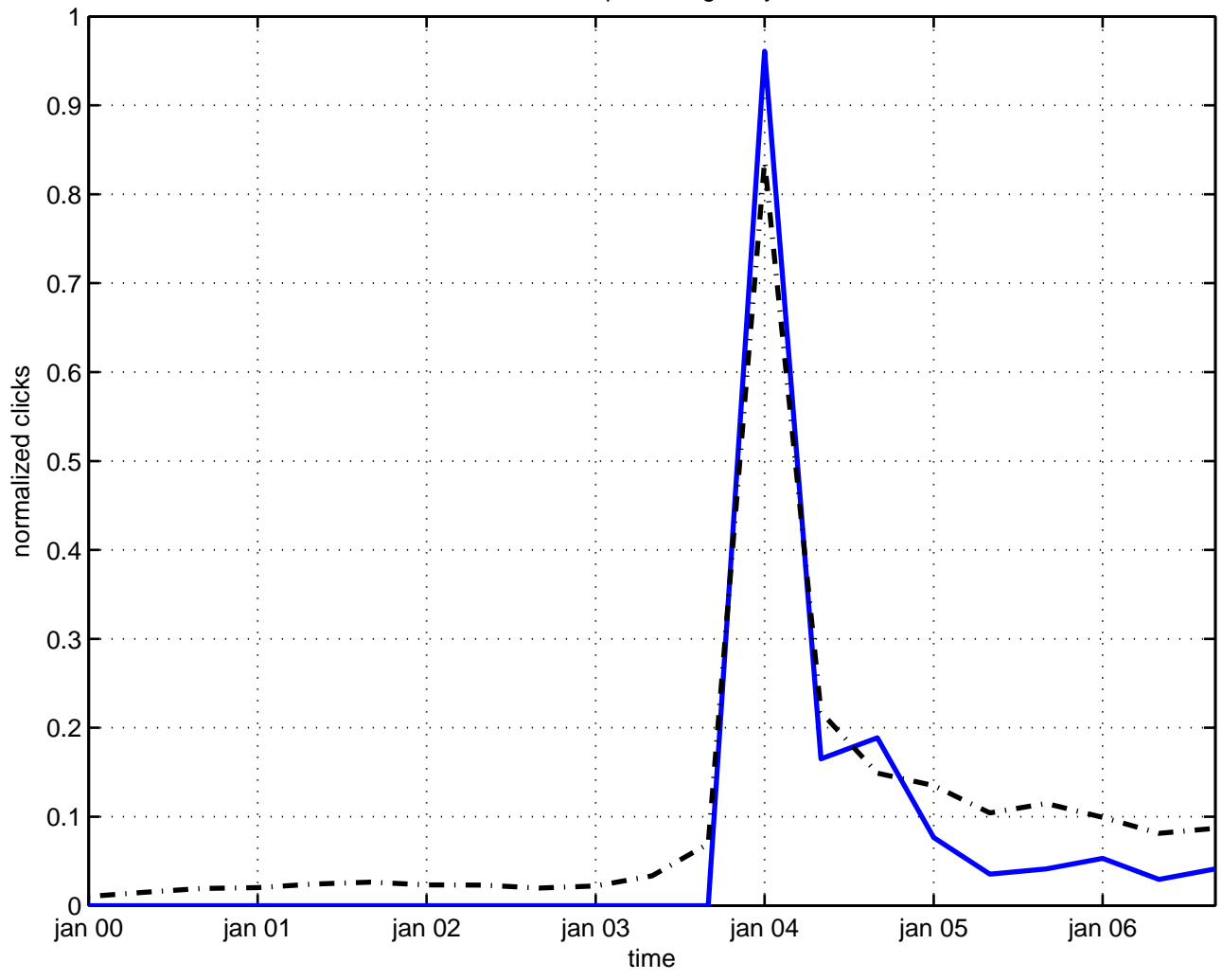
affine quantum gravity
