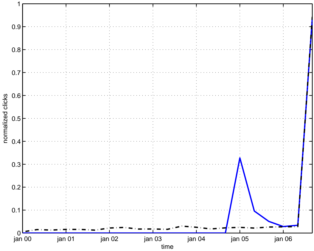
affine geometry
