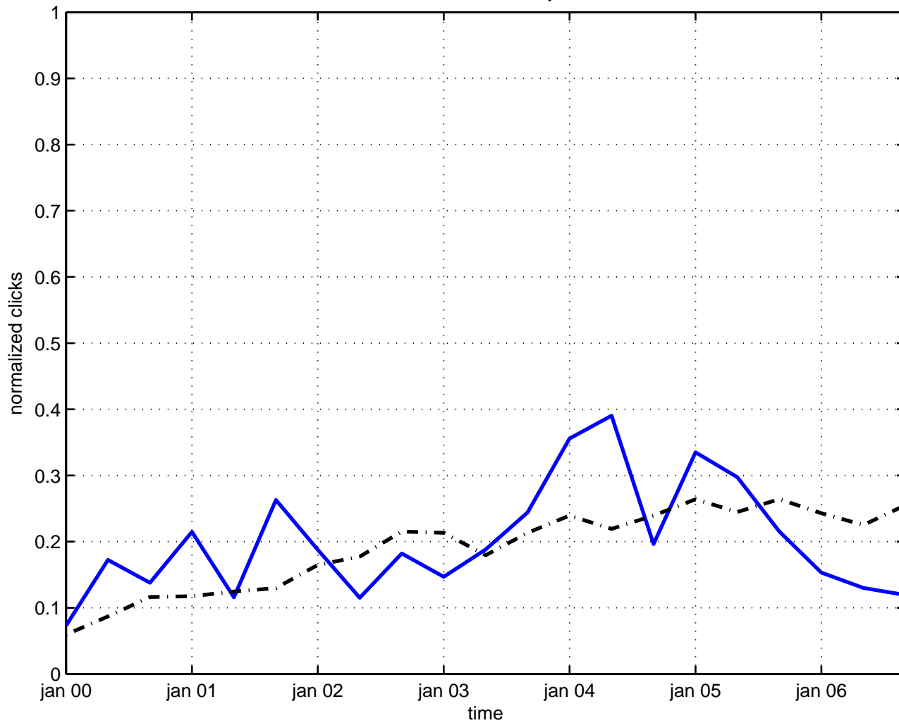
affine field theory
