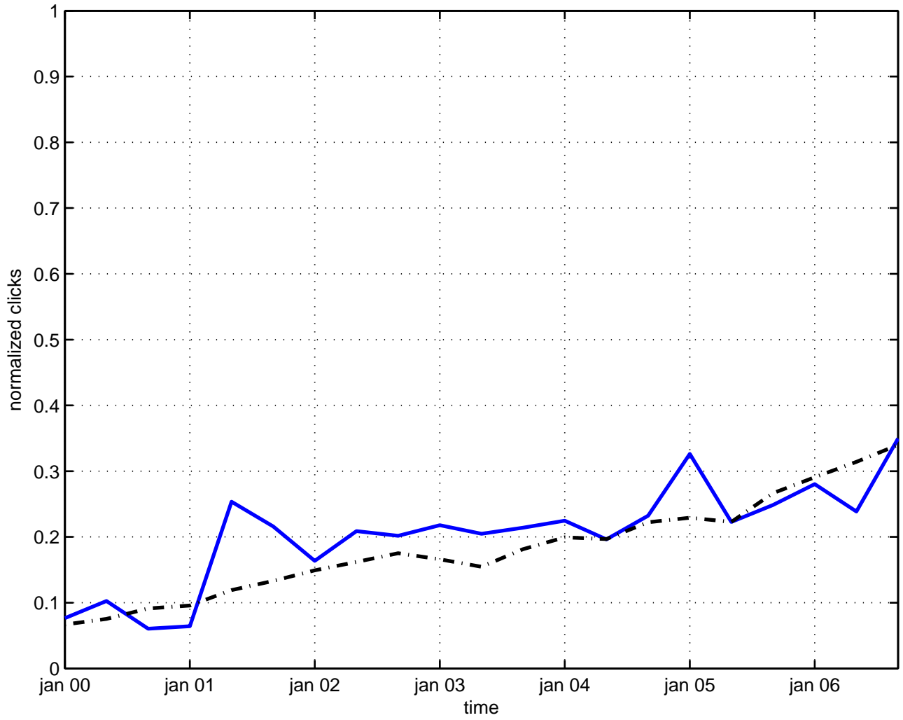
affine algebra
