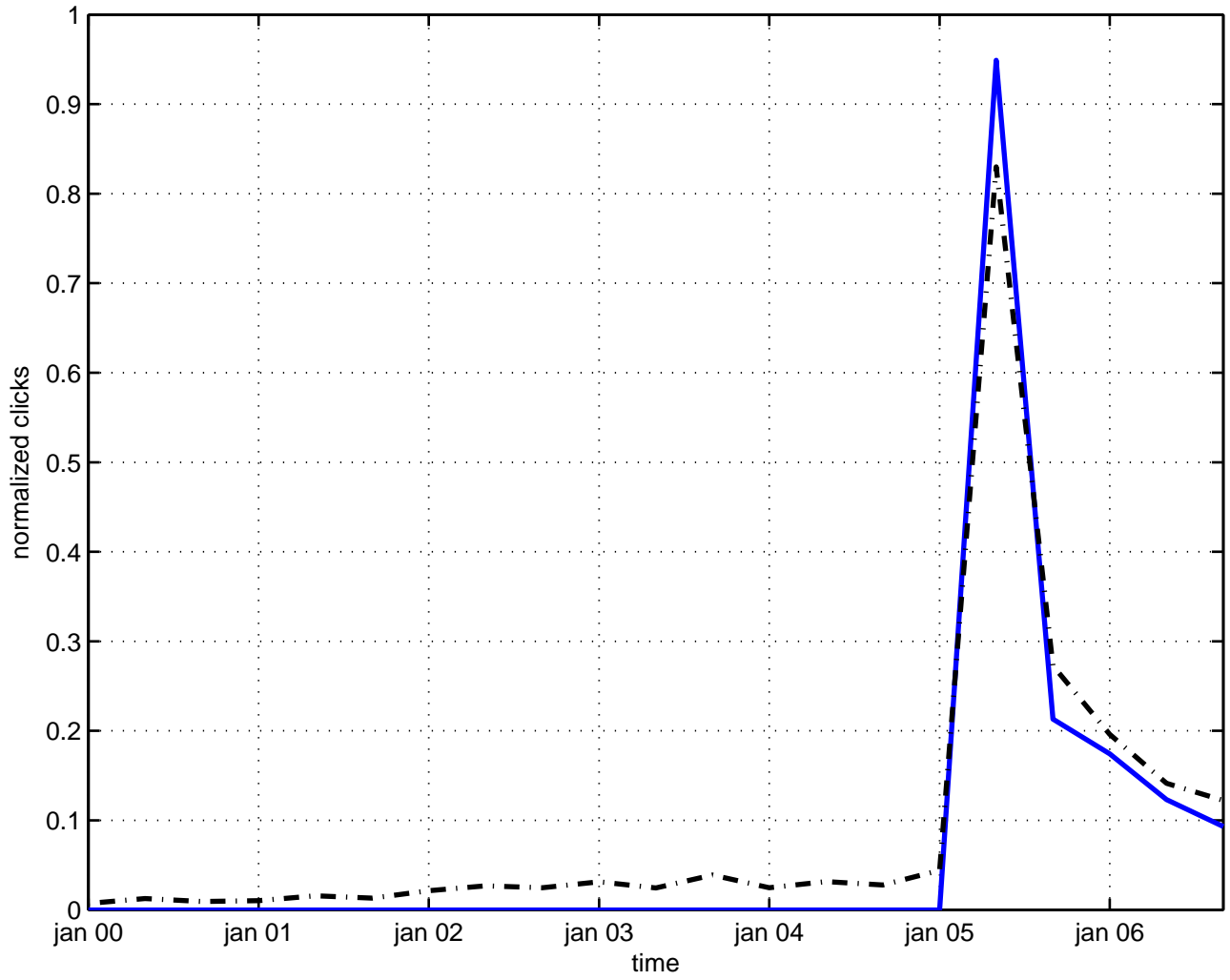
ads/cft correspondence
