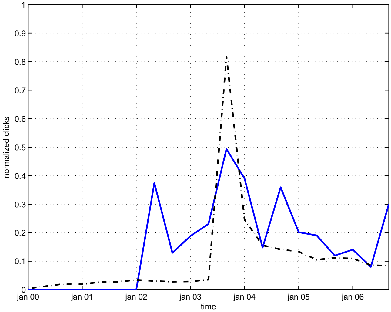
adiabatic perturbation
