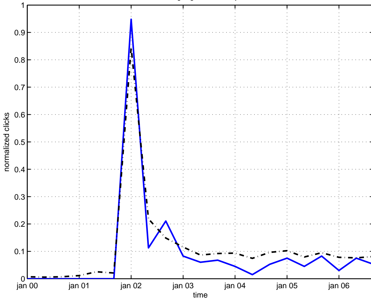
ade gauge field theory
