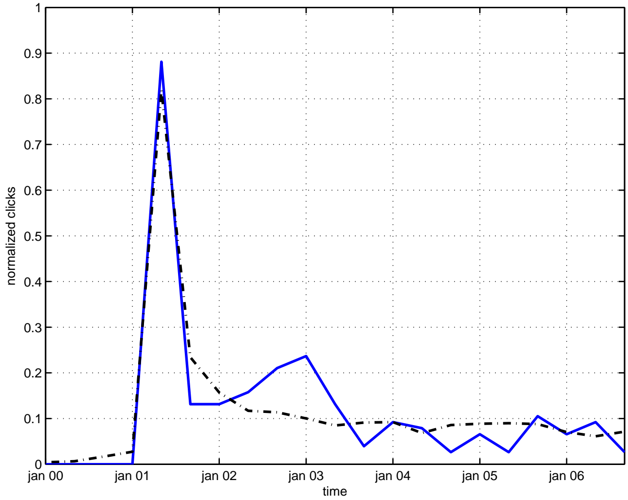
action sine-gordon model
