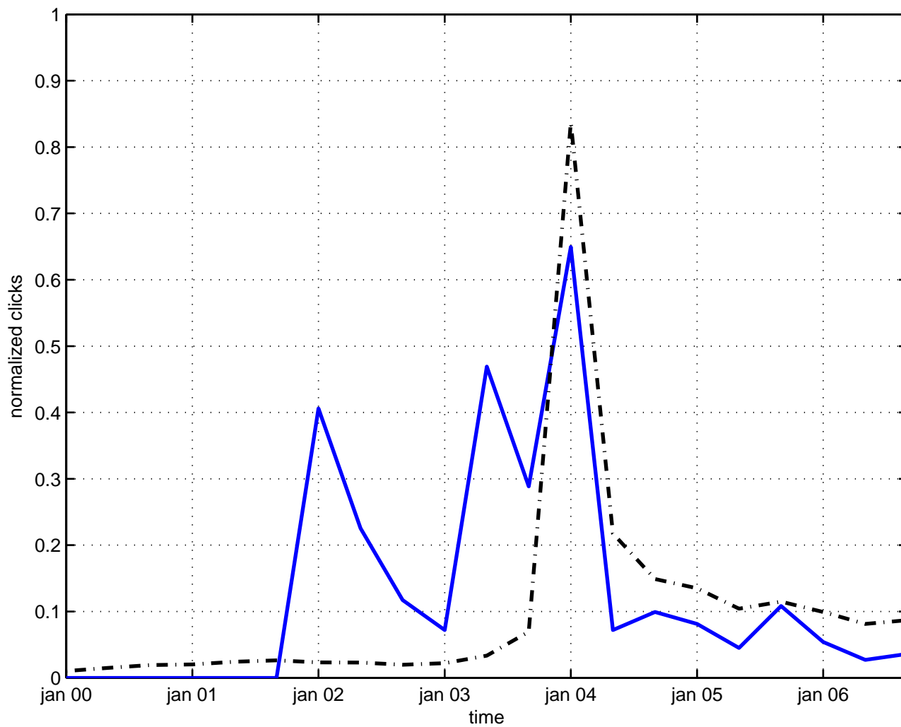
accretion matter
