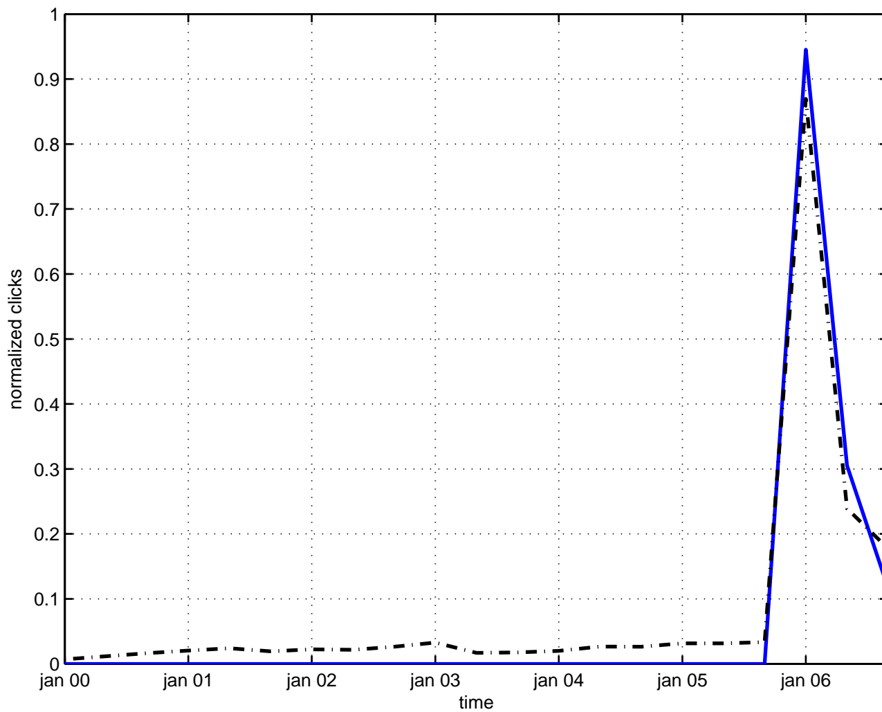
accretion black hole
