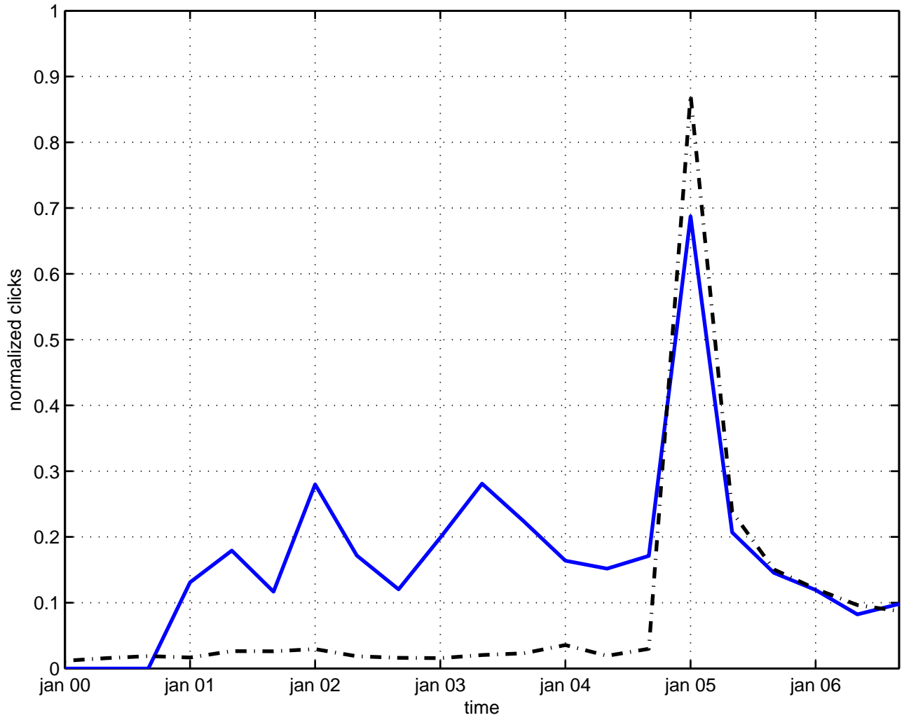
acceleration astrophysics
