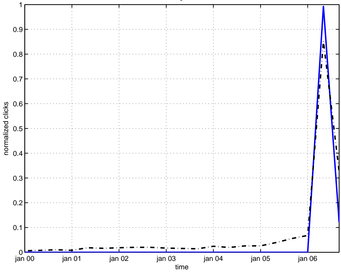
abelian sigma model
