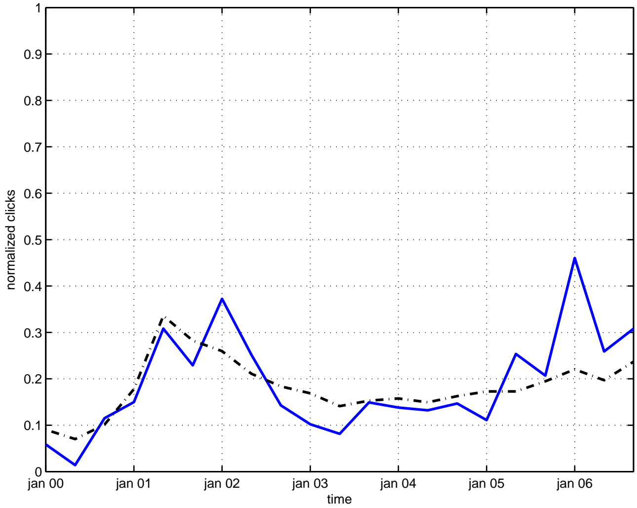
abelian higgs model
