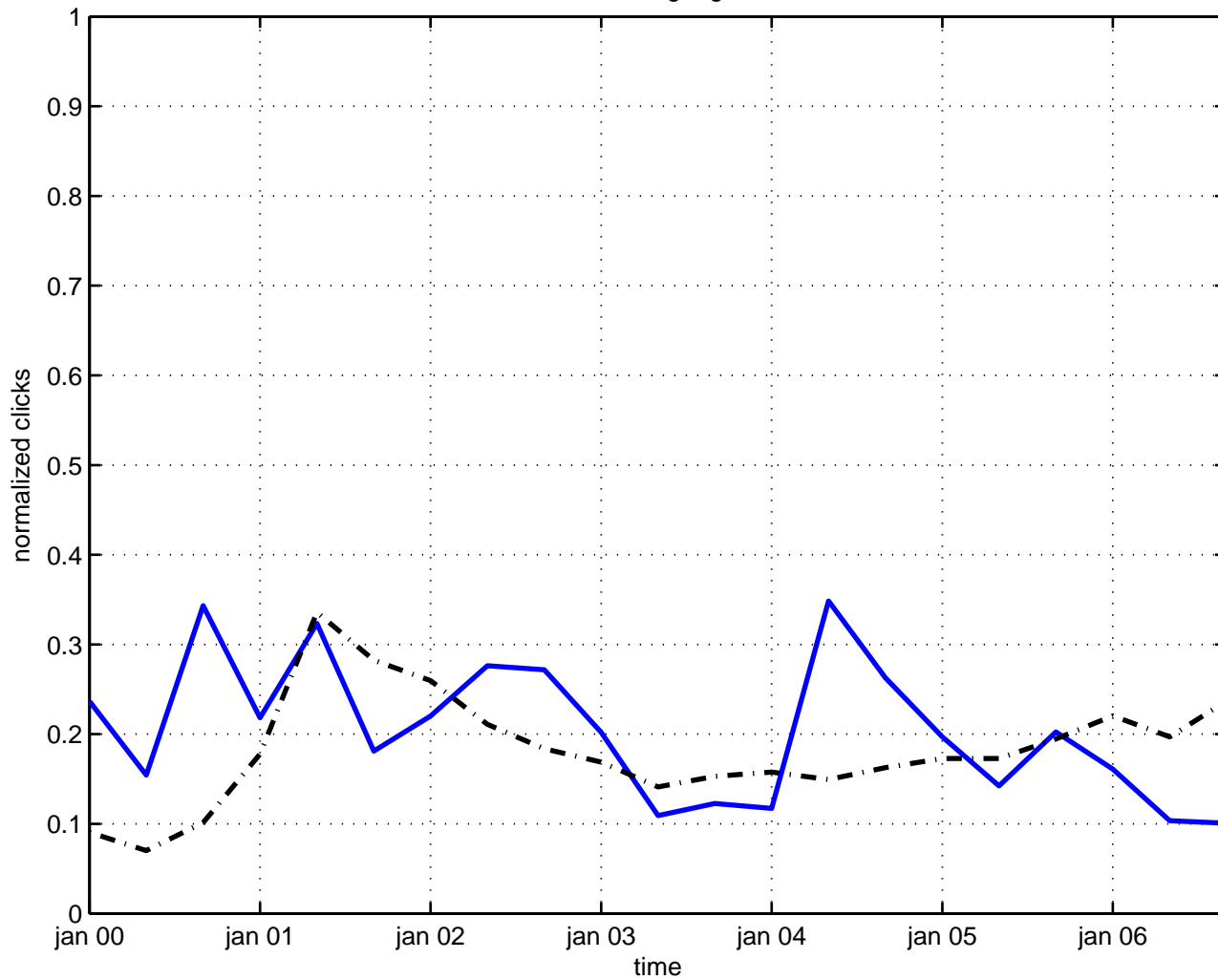
abelian gauge
