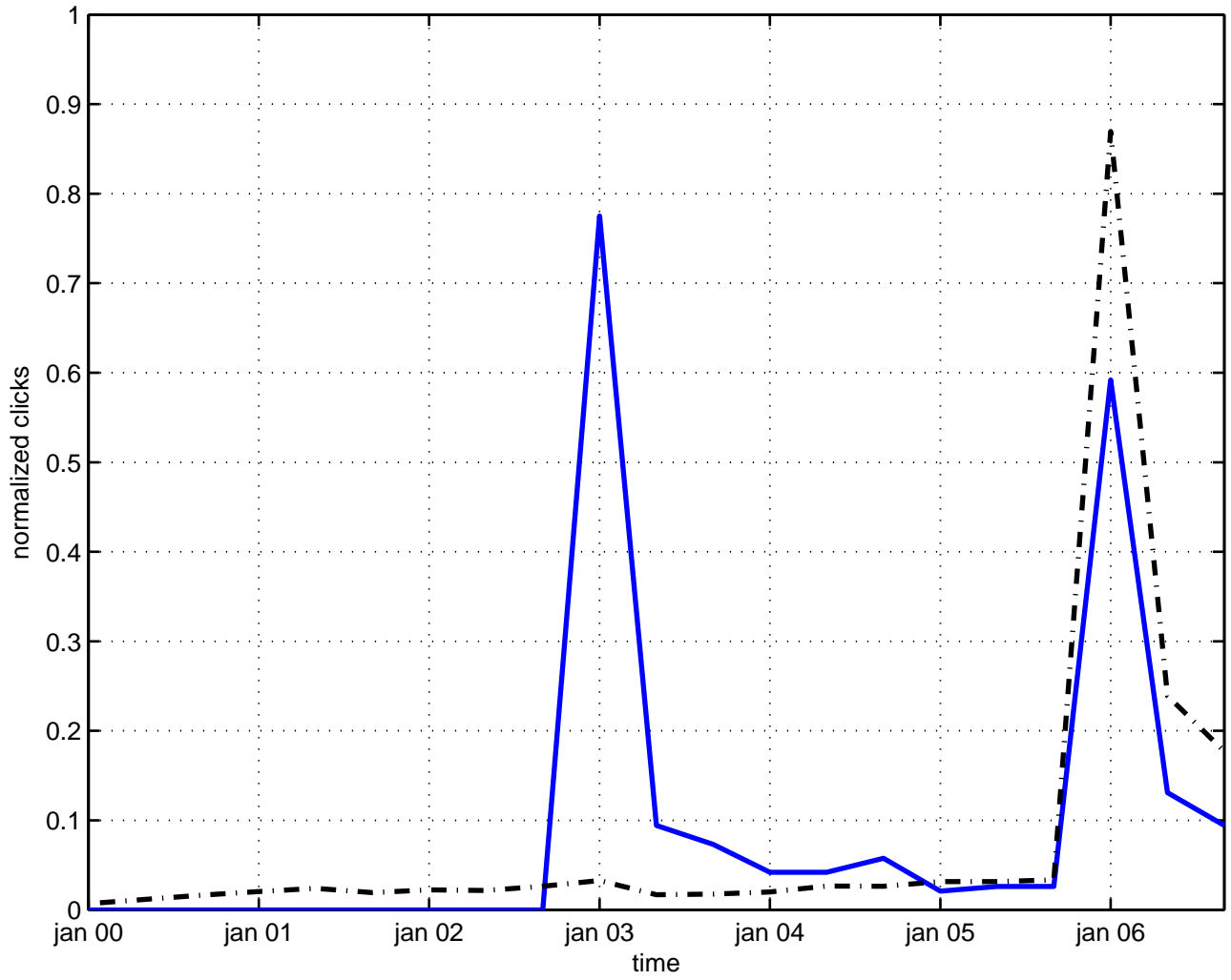
abelian embedding
