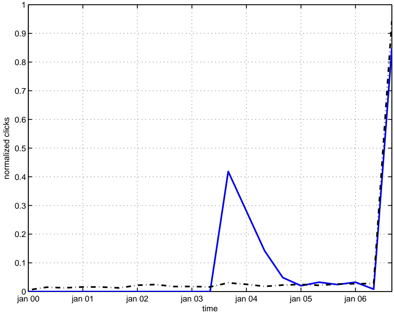
abelian duality
